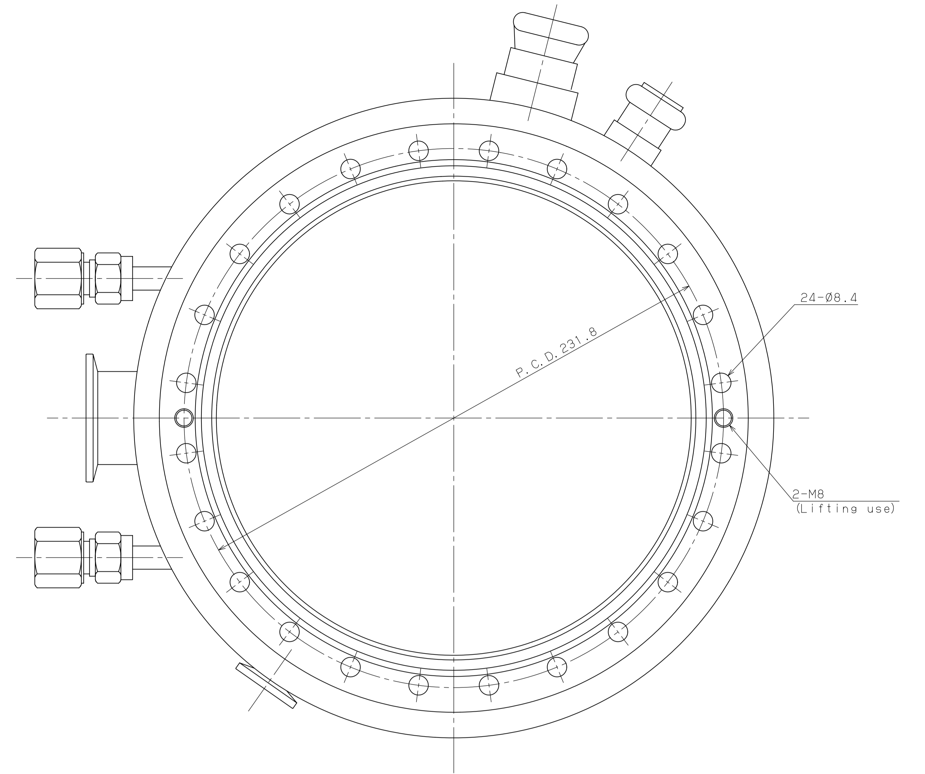
View "A"
