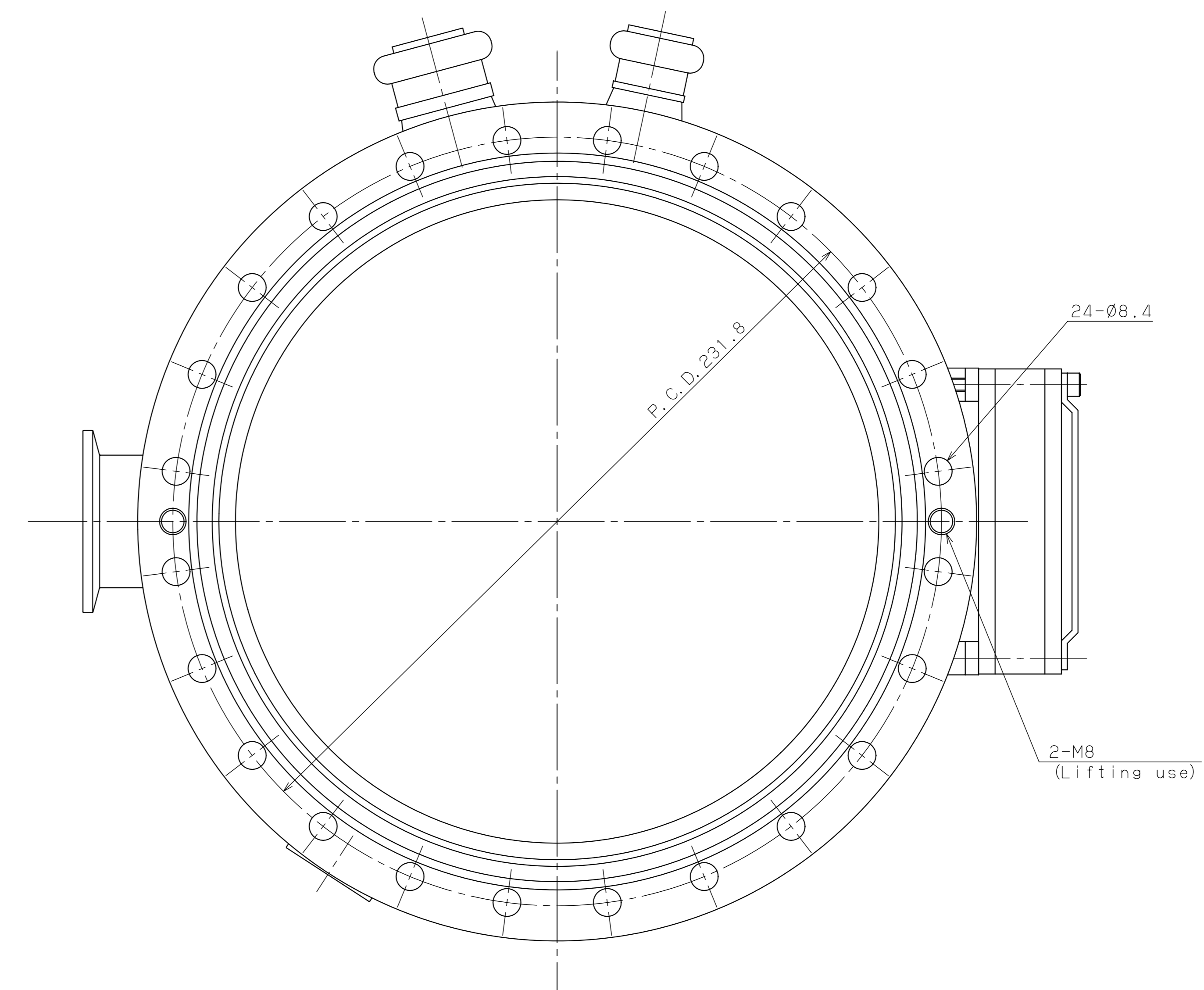
View "A"
