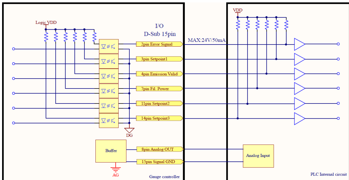
Figure 3-2 SH200-A output signal internal circuit diagram
