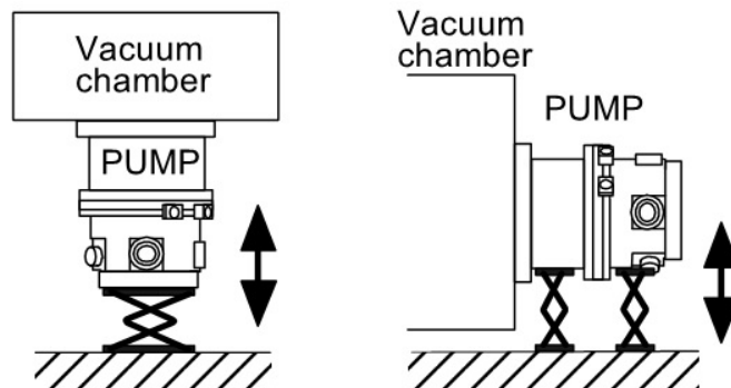
Fig. 5-2 Lifting Method
