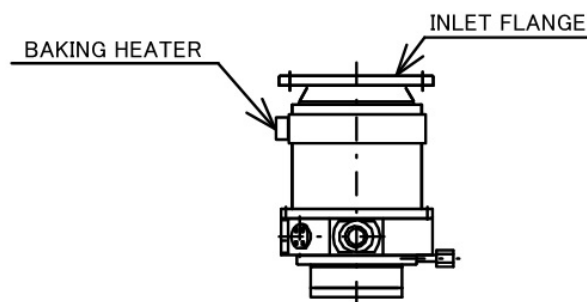
Fig. 6-1 Installation of Baking Heater
