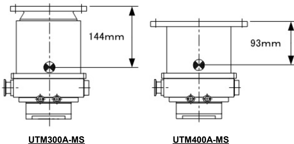
Fig. 5-7 Center of Gravity of the Pump
