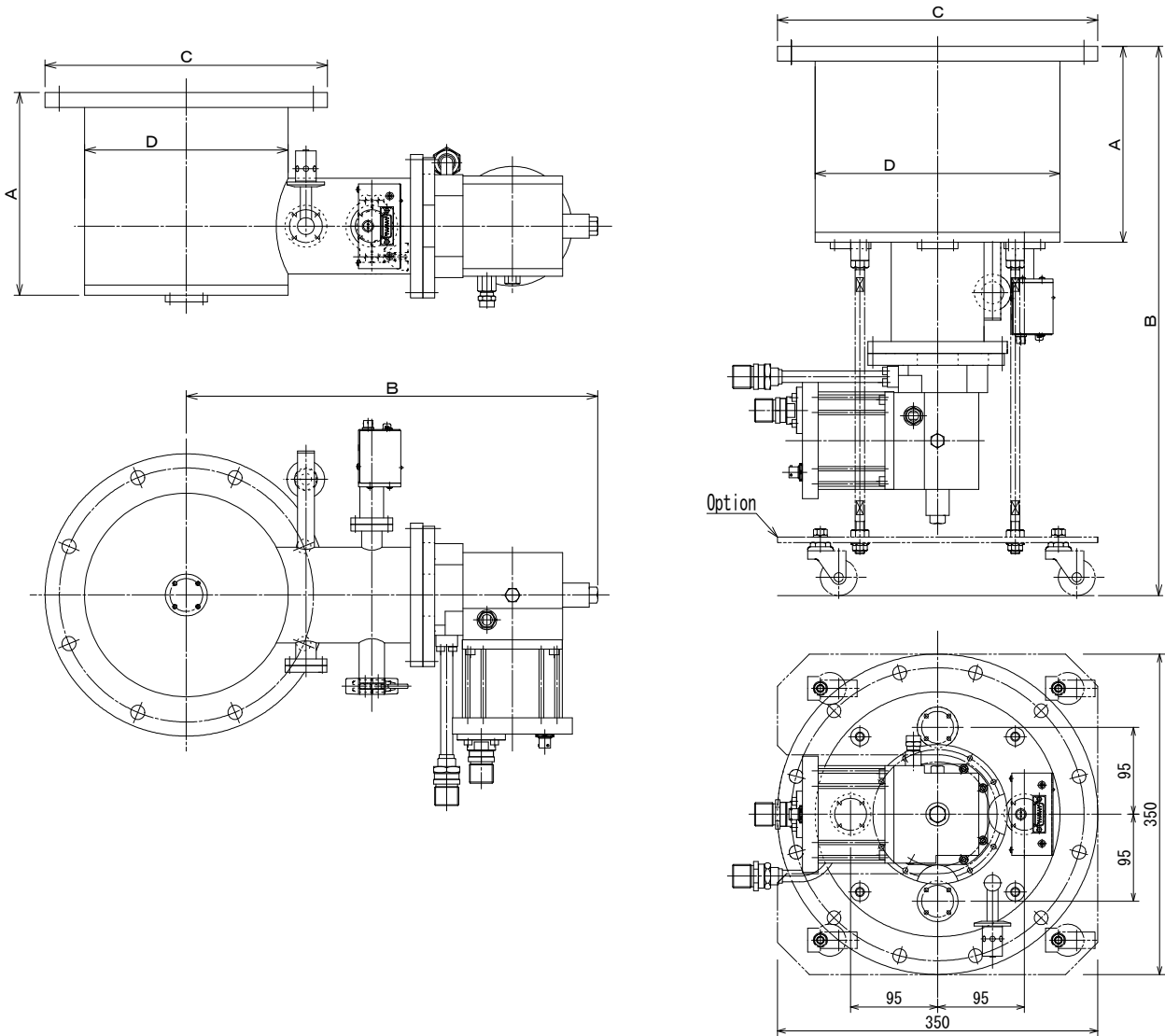
Figure 1-2 External Drawing of CRYO-U® Cryopump (Continued)
