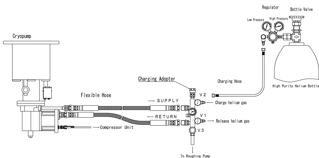
Figure 8-4 Cryopump Decontamination Procedure (1)
