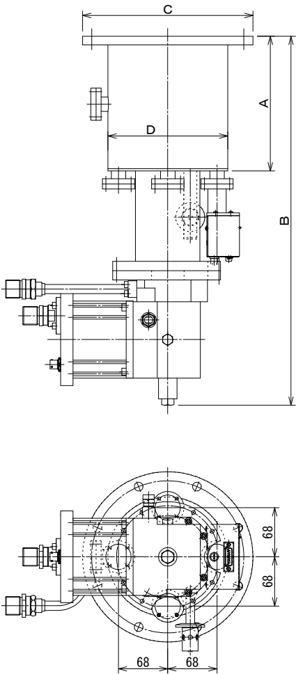
Figure 1-2 External Drawing of CRYO-U ® Cryopump
