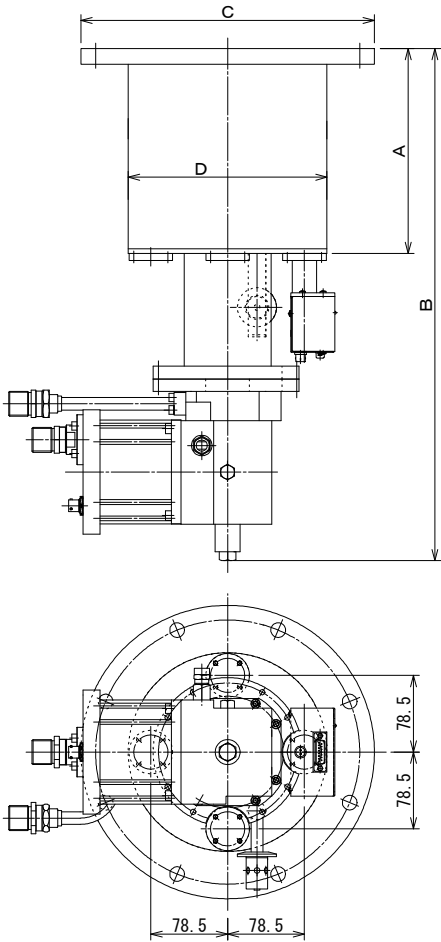
Figure 1-2 External Drawing of CRYO-U ® Cryopump
