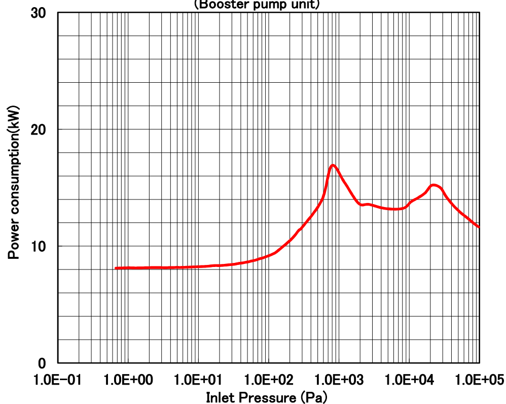
Power-Pressure curve (Booster pump unit)
