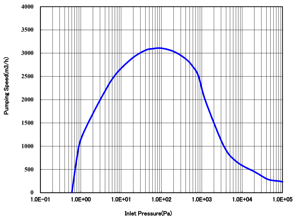
Pumping Speed (Booster pump unit)
