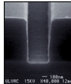
GaAs/AlGaAs selective Etching (anisotropic)
