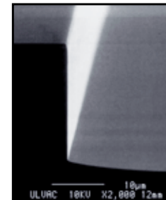
GaAs/AlGaAs non-selective Etching
