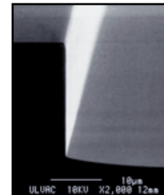
GaAs/AlGaAs non-selective Etching
